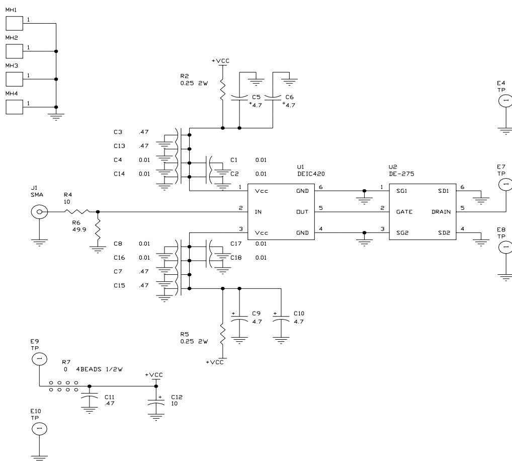
Figure 17 - High Frequency Gate Drive Circuit
