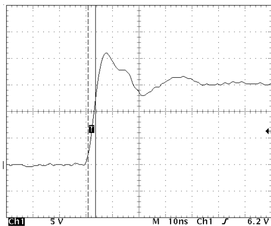
Figure 11 3ns Rise Time
