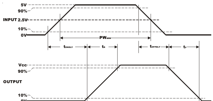
Figure 3b - Timing Diagram
