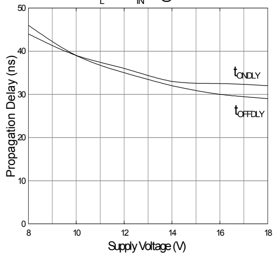
Fig. 10 Propagation Delay vs. Supply Voltage C_L = 4\text{nF} V_{IN} = 5\text{V}@100\text{kHz}
