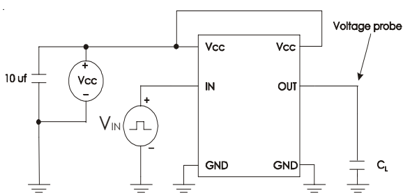
Figure 3a - Characteristics Test Diagram
